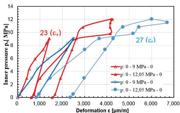
Figure 4 Strain change with pressure in welded joint LS4, for strain gauges 27 ( \epsilon_t ) and 23 ( \epsilon_z )
