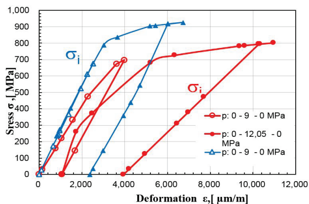
Figure 3 Stress strain diagram for the parent material
