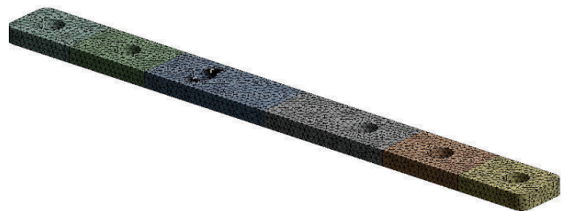
Figure 6 Plate A mesh with initial cracks
