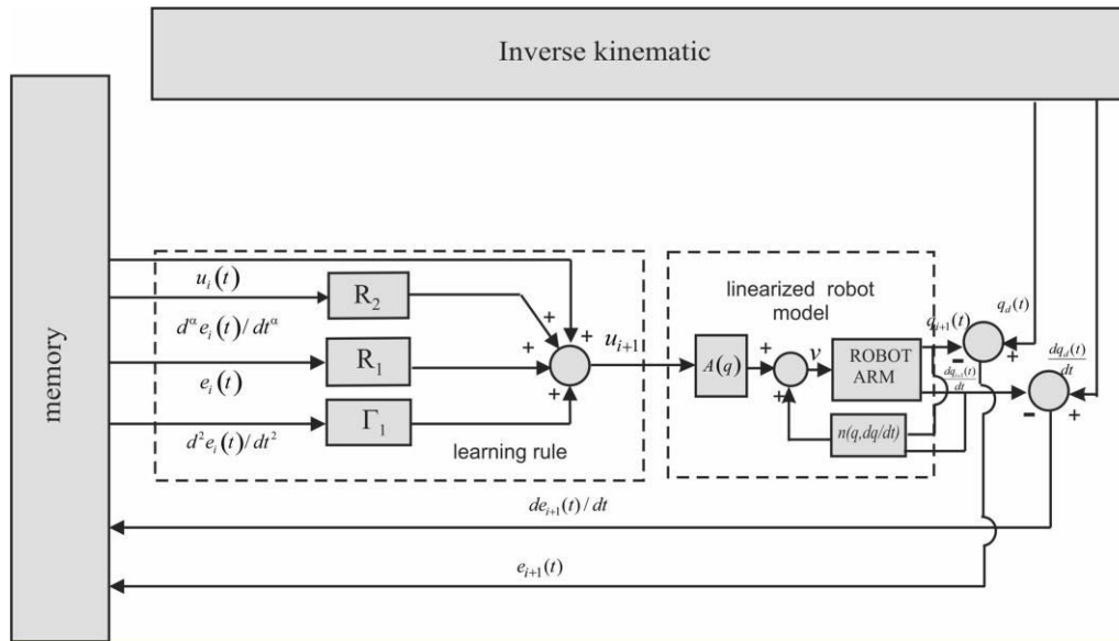
Figure 1: Block diagram of the open-loop PD^2D^\alpha law for the robot control
